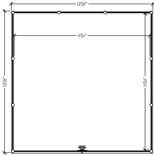
PLAN 10' x 10'
